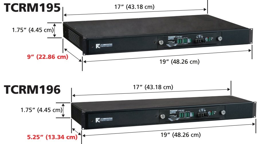
TCRM195/196 rack mount card cage (shown with optional built-in power supply)
