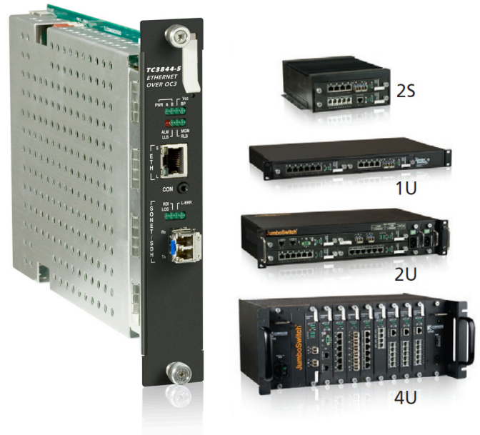
TC3844-5 Ethernet-over-OC-3/STM-1 Gateway
