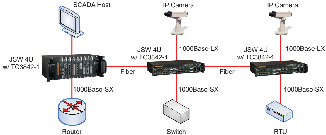
Application Using TC3842-1 to Extend the Existing Gigabit Ethernet Network to the Remote Sites
