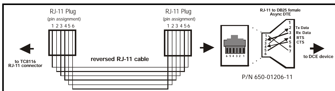
Figure 11. RJ-11 (ASYNC DTE) Pin Assignments & Connection
