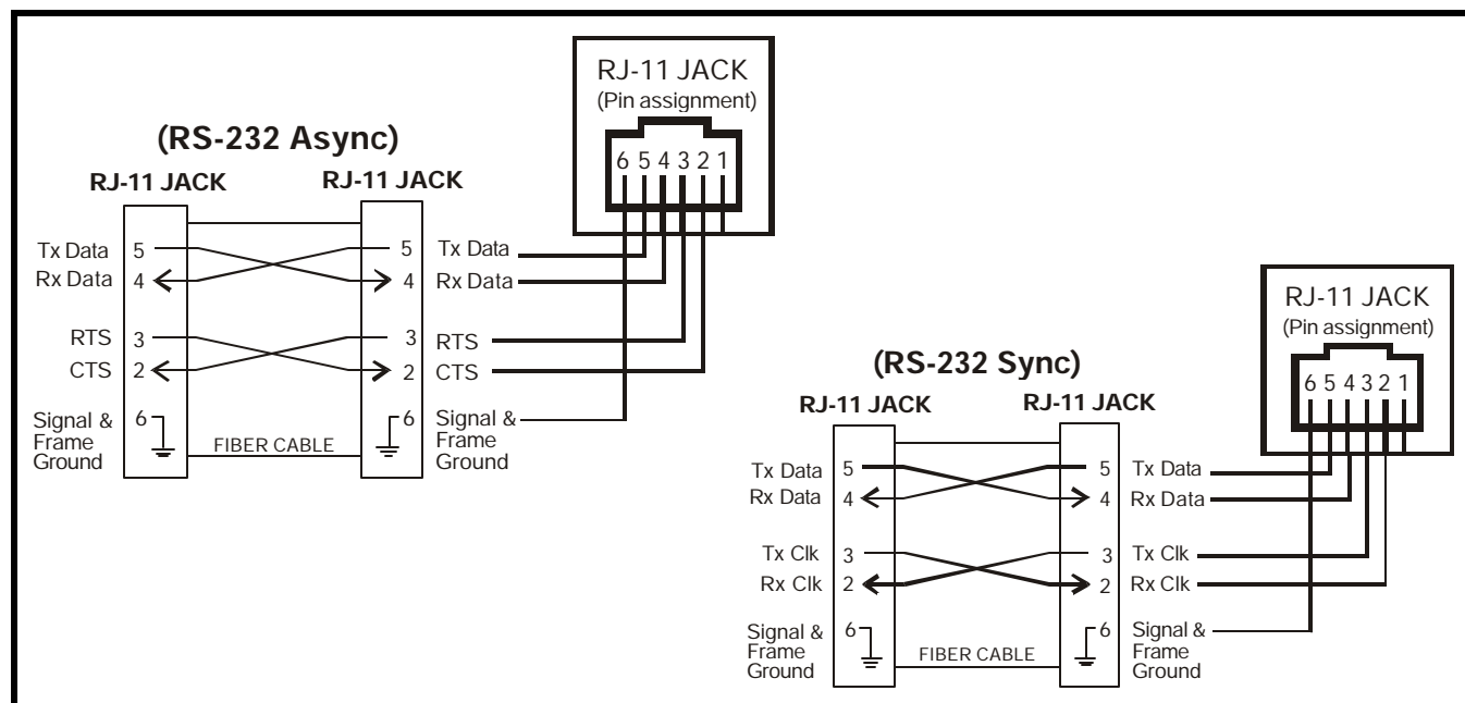
Figure 4. RS-232 Async Pin Assignments & Virtual Connection Diagram
