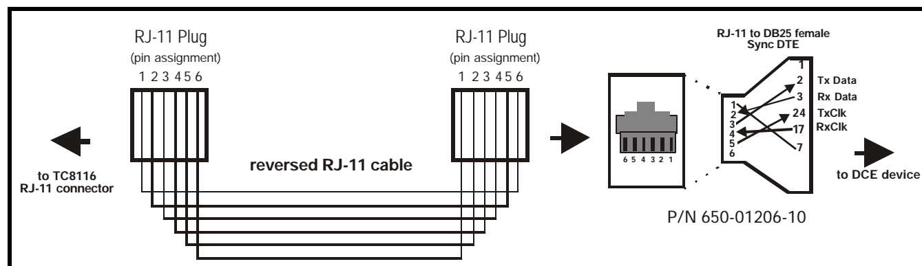
Figure 13. RJ-11 (SYNC DTE) Pin Assignments & Connection
