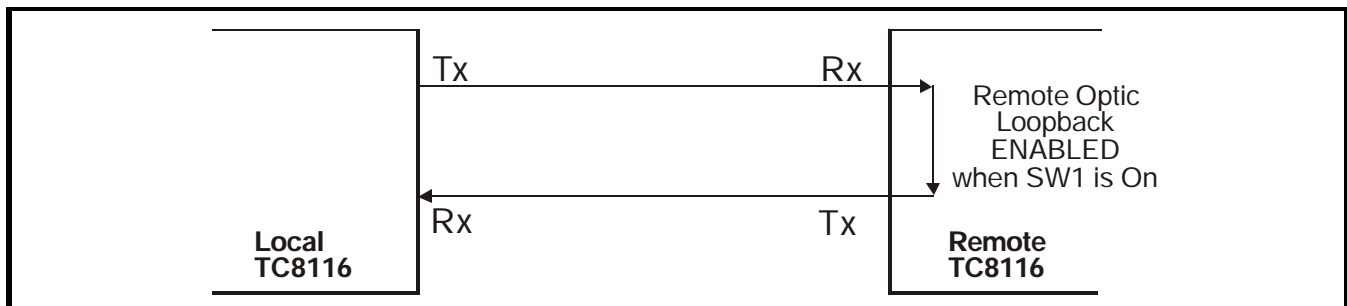
Figure 17. Remote Loopback Logic Diagram
