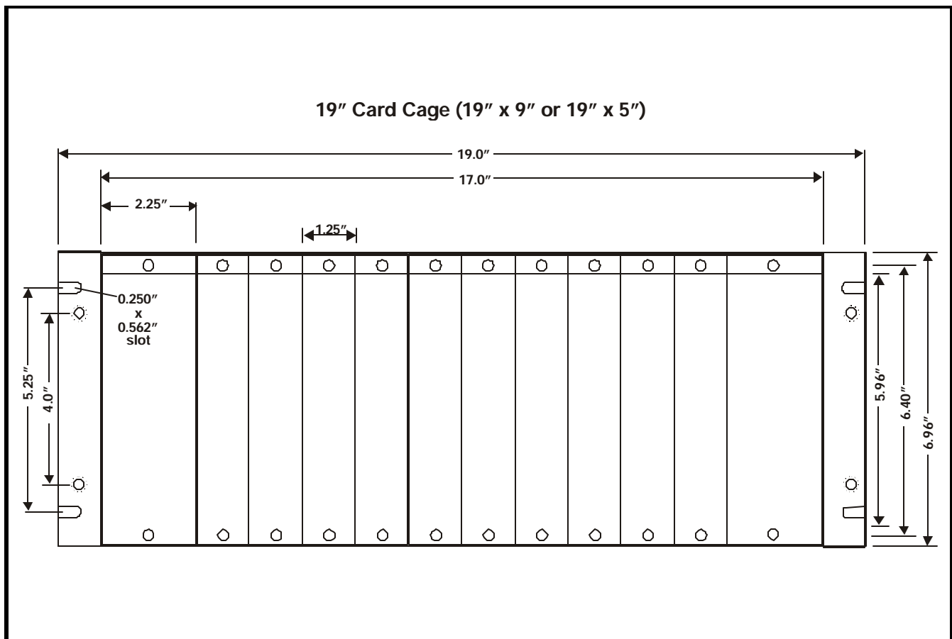
Figure 18. TCRM191/192 Rack Mount Card Cage
