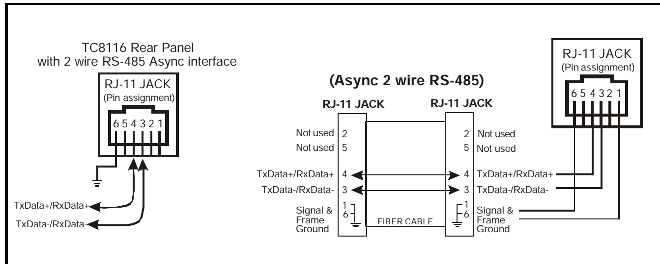
Figure 6. Two wire RS-485 Async Pin Assignments & Virtual Connection Diagrams
