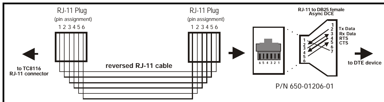
Figure 10. RJ-11 (ASYNC DCE) Pin Assignments & Connection
