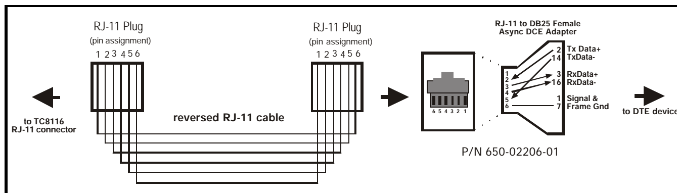
Figure 14. RJ-11 (ASYNC DCE) RS-422/RS-485 Pin Assignments & Connection
