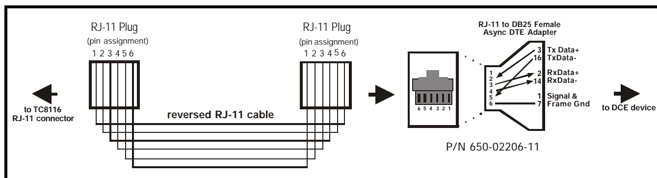
Figure 15. RJ-11 (ASYNC DTE) RS-422/RS-485 Pin Assignments & Connection
