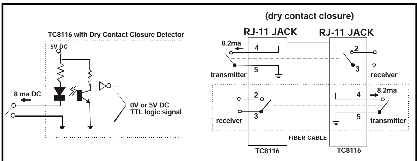
Figure 9. Dry Contact Detector and Closure Logic Diagrams
