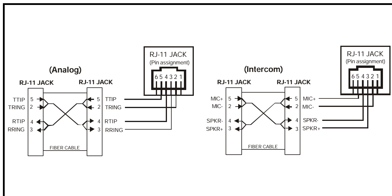
Figure 7. RJ-11 Analog and Intercom Pin Assignments & Virtual Connection Diagrams
