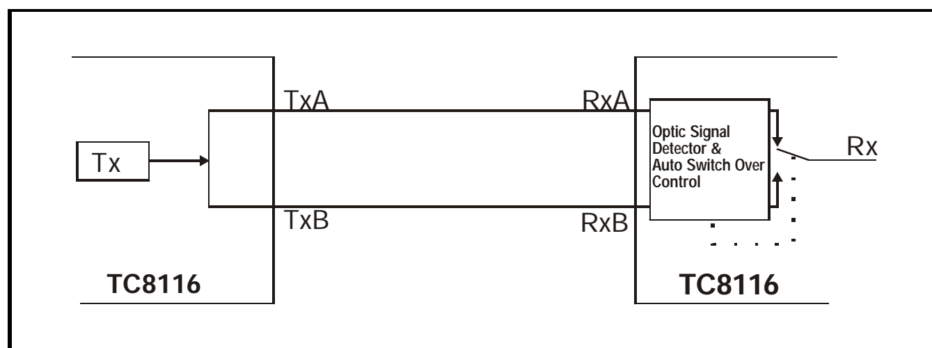
Figure 16. Dual Optics Logic Diagram
