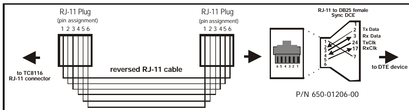
Figure 12. RJ-11 (SYNC DCE) Pin Assignments & Connection
