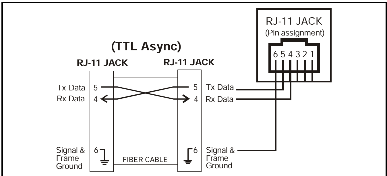
Figure 8. RJ-11 TTL Async Pin Assignments & Connection Diagram
