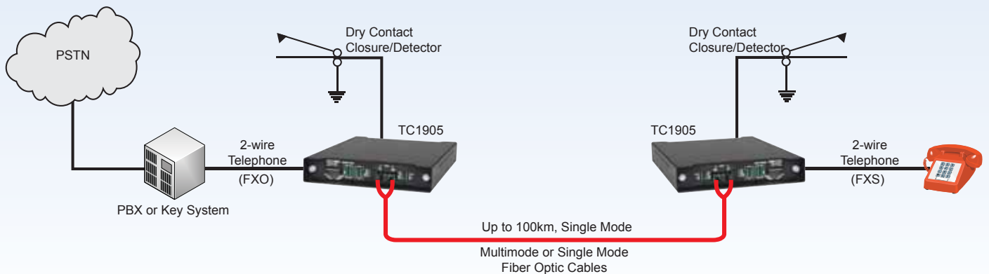
Typical Point-to-Point Application Using TC1905s to Extend Telephone and Dry Contact via Fiber Optic Cables
